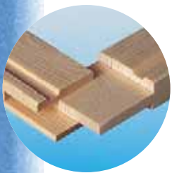
Wood joints are mortised and tenoned, glued and stapled
