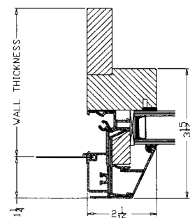
Direct set fixed window jamb detail
